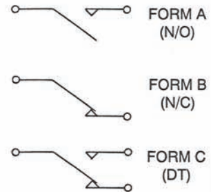
Figure 1b. Contact Forms
