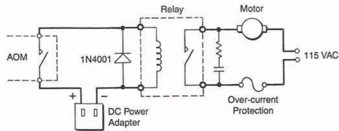
Figure 2b. Alarm Output (AOM) Motor-control Circuit.
