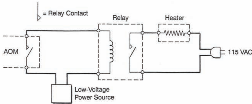
Figure 1a. Use of a Relay to Switch a Heater. (Simplified circuit.)
