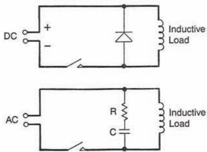
Figure 2a. DC Circuit with Diode Clamp. AC Circuit with Snubber.
